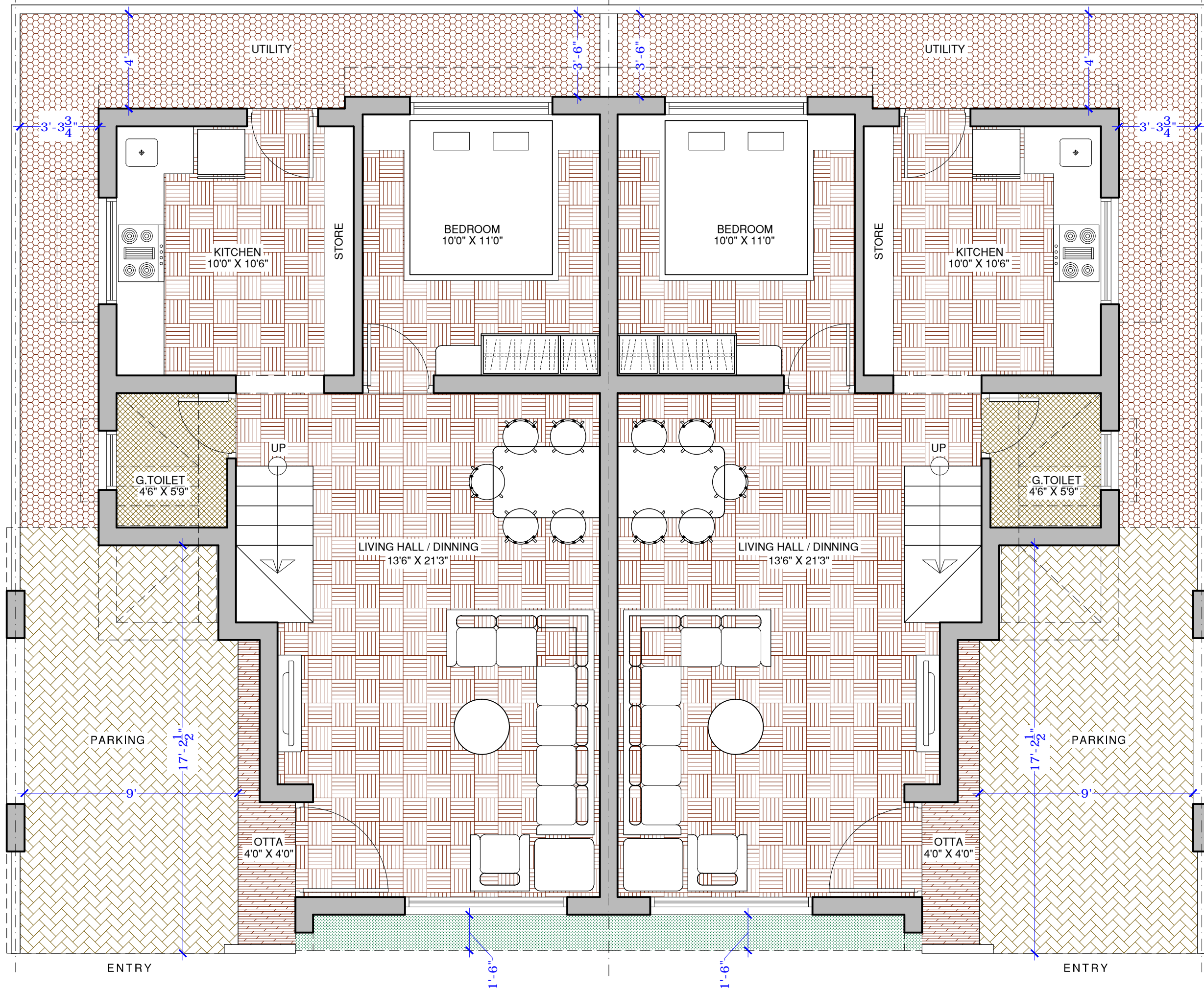
DRAWING : GROUND FLOOR PLAN - 862 SQ.FT. AREA
